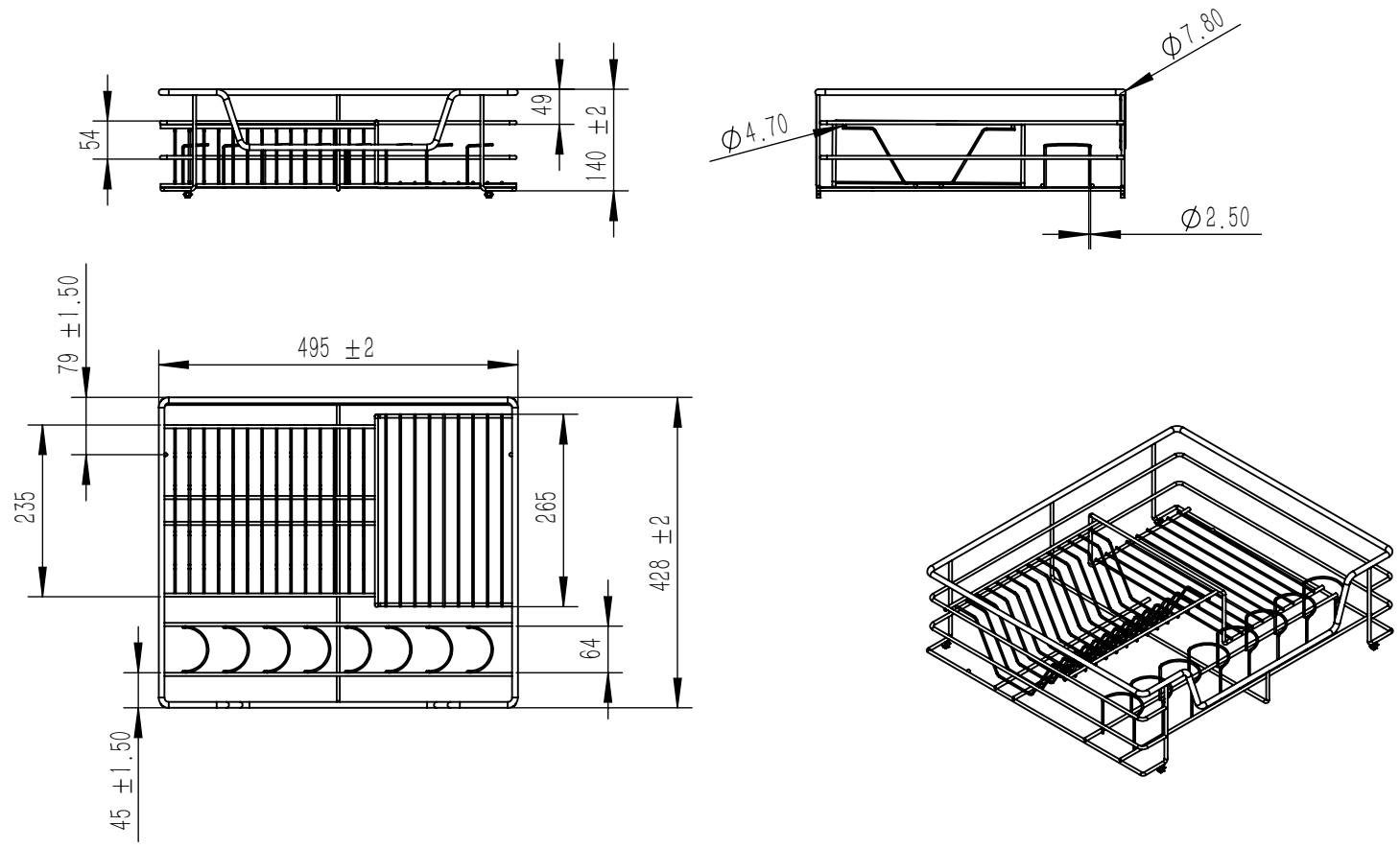
14.01.231 4-Side Pull-Out Basket
